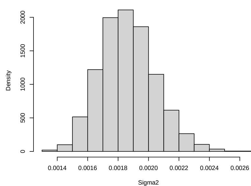
Density of Sigma2
